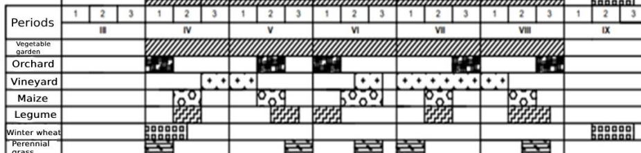
Graph 4. Completed water duty graph
