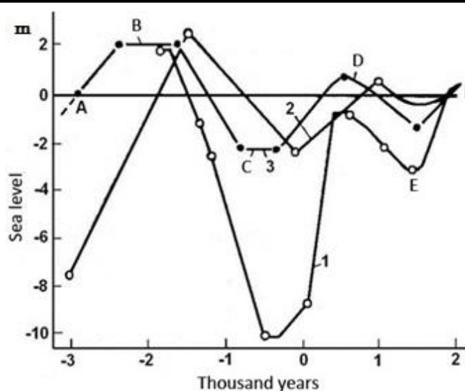
Fig 1. Water level fluctuations in the Black Sea over the past 5000 years
