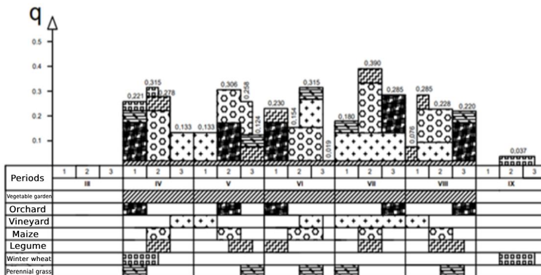
Graph 5. Completed water duty graph including water demand curve
