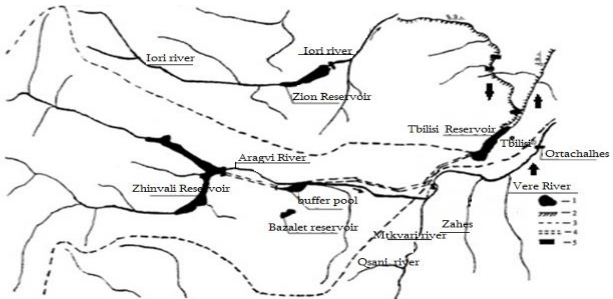
Fig. 1. Joint operation scheme of Sion, Tbilisi and Zhinvali reservoirs
