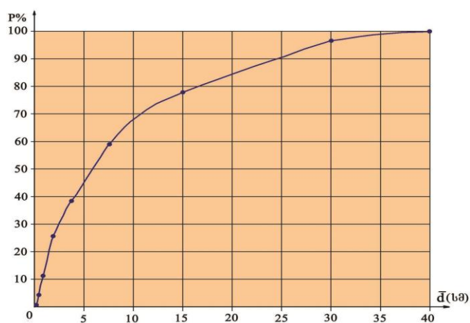
Fig. 3. Integral curve of granulometry of the first sample
